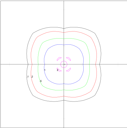
Type V • 7023 Lumens Maximum Calculated Value: 2.17 Fc
