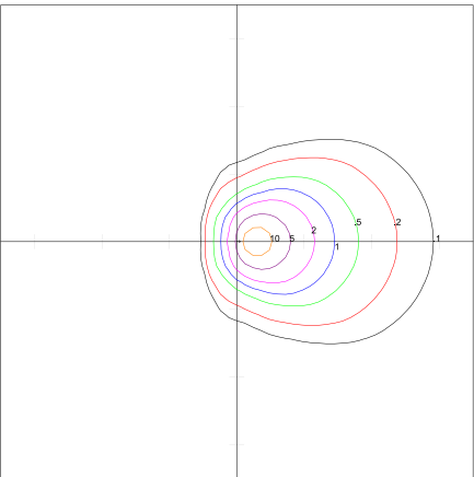
70° Optics • 7408 Lumens Maximum Calculated Value = 14.04 Fc
