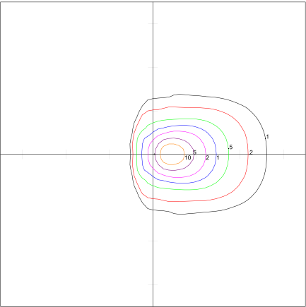
40° Optics • 7249 Lumens Maximum Calculated Value = 18.83 Fc
