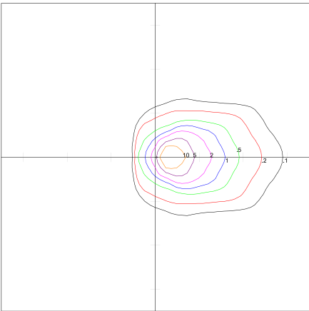
55° Optics • 7269 Lumens Maximum Calculated Value = 19.14 Fc
